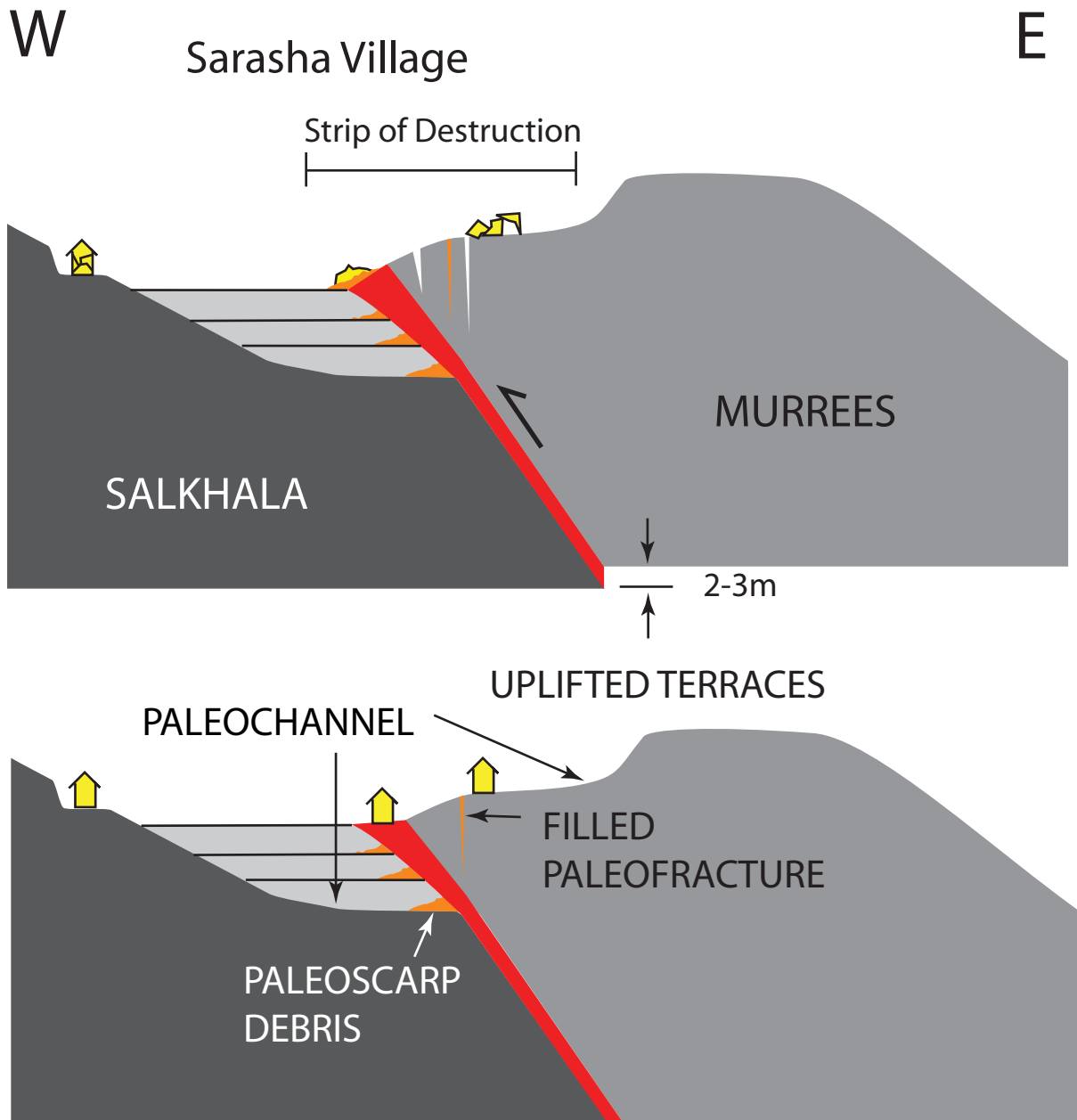
Hypothetical section through the October 2005 rupture in Sarasha Village based on surface observations of the landform changes caused by the 2004 thrust-fault rupture. Current geomorphic setting of the location is a saddle.
